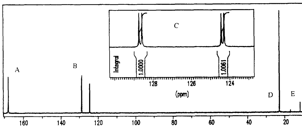
Figure ^{31}\text{P}\{^1\text{H}\} NMR of 5f ; in ppm. A = unreacted 3 ; B = P(III) resonances of 5f x and 5f y ; C = expansion of B (data collected as described in reference 9); D = P(V) resonances of 5f x and 5f y ; E = 4 caused by trace hydrolysis of 3 .
